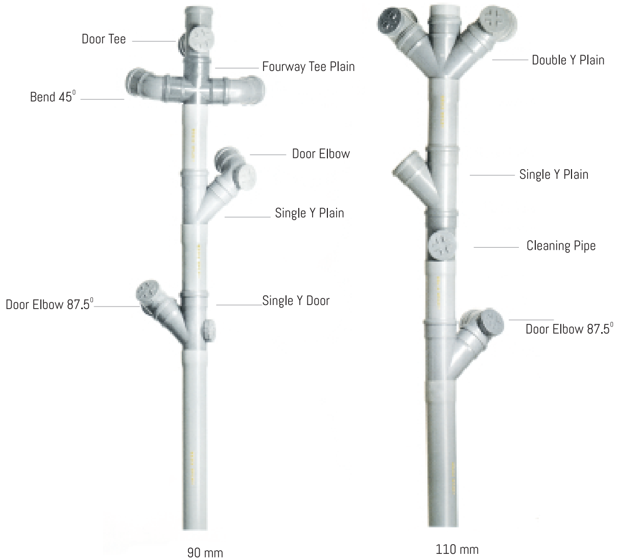
Typical Sanitation System
